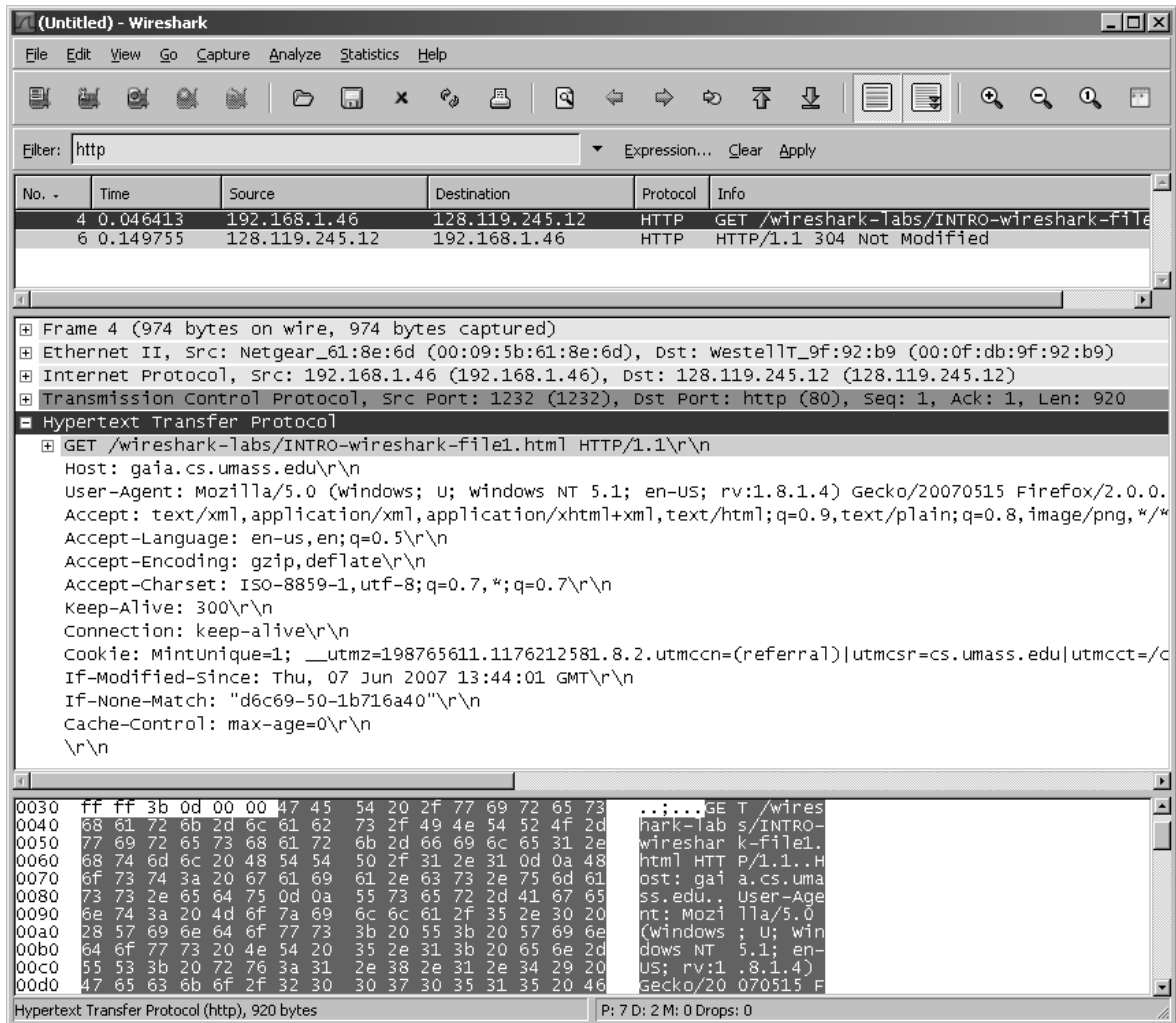
Figure 5: Wireshark display after step 9
